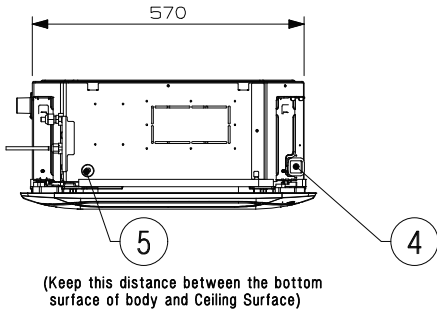
Installation position of body
