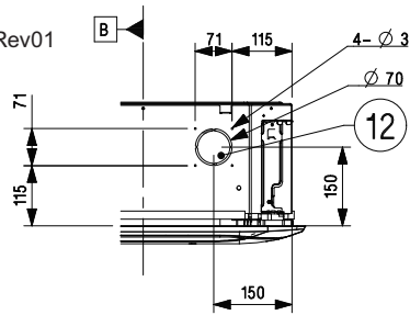
View A Fresh Air Intake hole
