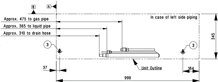
Connecting gas/liquid pipe, drain hose
