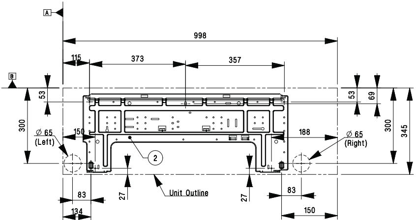
Fixing the installation plate, drilling hole
