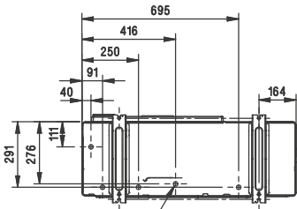
5-I.D. 20 holes for drain connection
