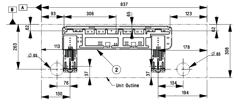
Fixing the installation plate, drilling hole
