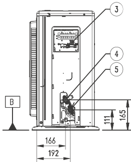
Side View (removed valve cover)
