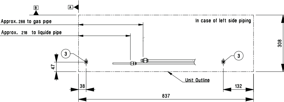
Connecting gas/liquid pipe
