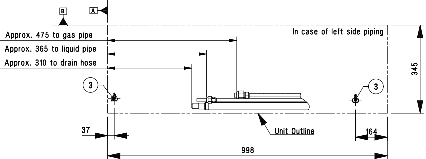
Connecting gas/liquid pipe, drain hose
